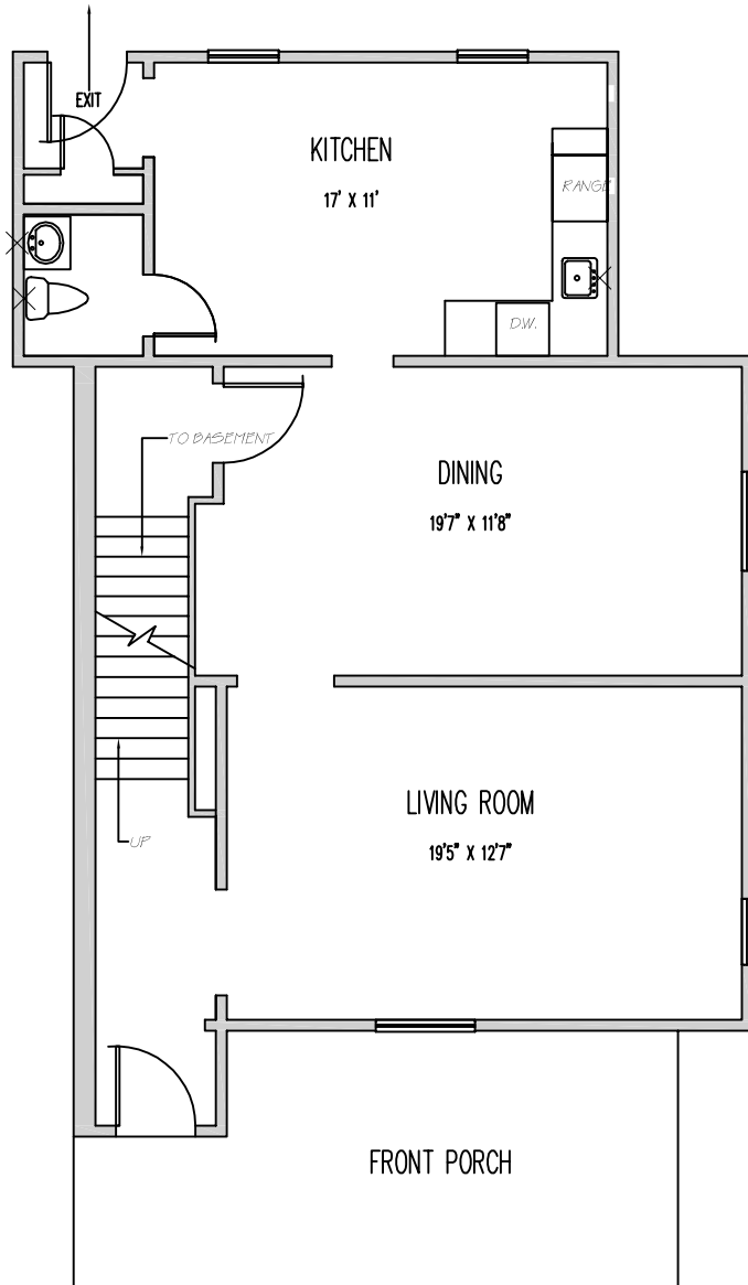
FIRST FLOOR
